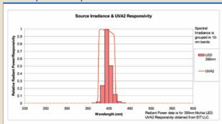
Spectral output of a 395 nm LED source and EIT UV-A2 spectral response
